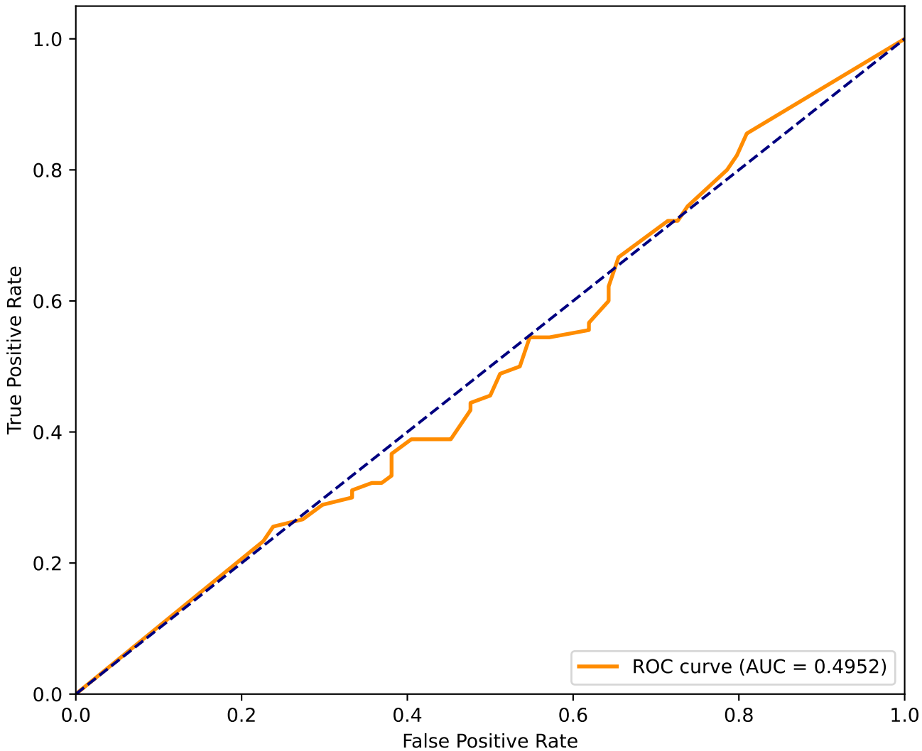
ROC Curve - DecisionTree
